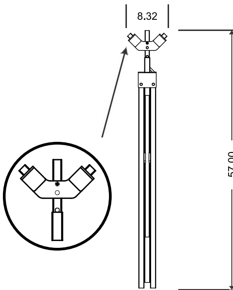
STORAGE DIMENSIONS
