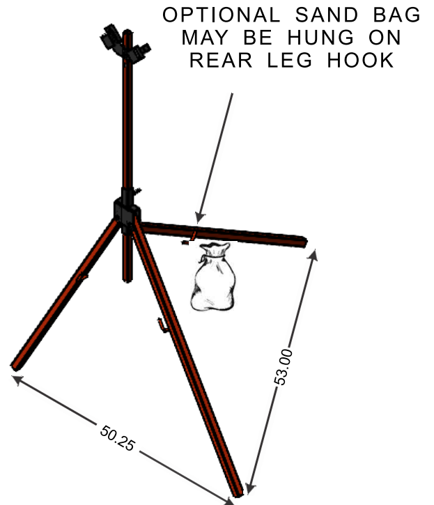
OPEN FOOTPRINT
